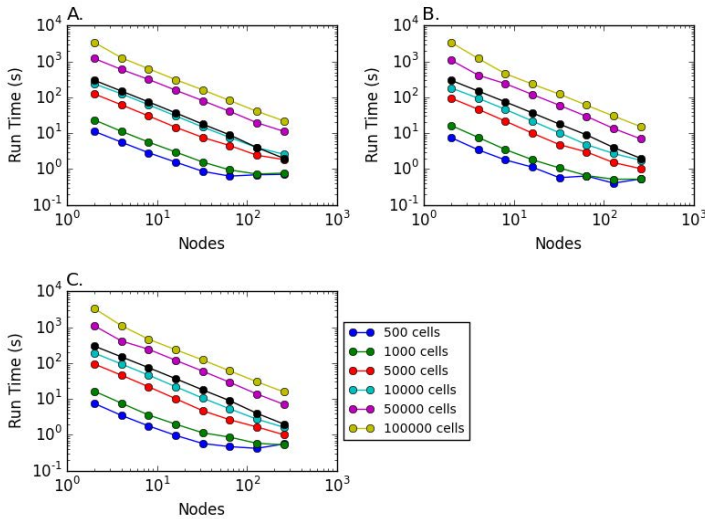
Figure 3: Simulation run time as a function of number of cells and number of nodes in log-log plots. (A) HH network. (B) I&F network. (C) Hybrid network. Black: linear reference.
